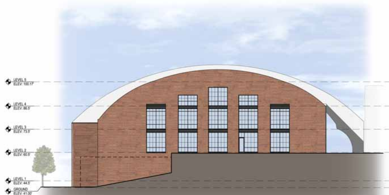
ELEVATION SOUTH: ARENA
