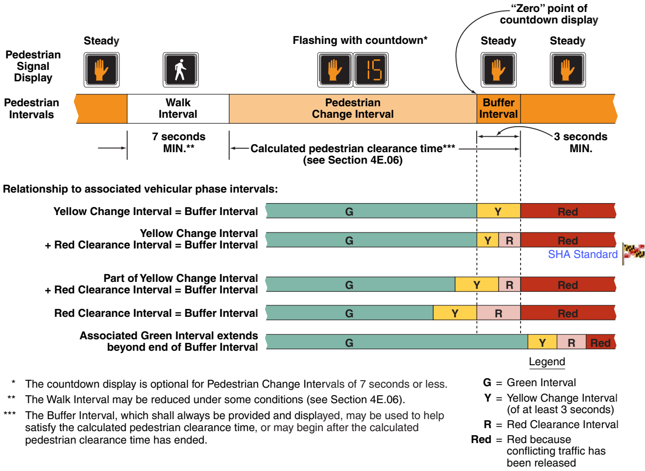
Figure 4. Pedestrian Intervals
